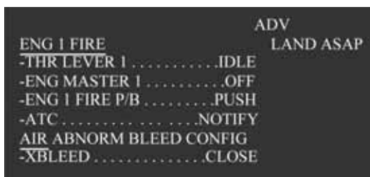
Figure 4. A version of the lower section of the ECAM display from an Airbus A330 aircraft with the text retained, but the colours removed. (Devised by Author 2)
